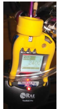
A CO 2 monitor reads concentrations in a swine barn.
